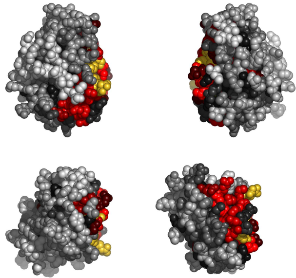
Fig. 2. Residues in 3borA, colored by their relative importance. Clockwise: front, back, top and bottom views.
