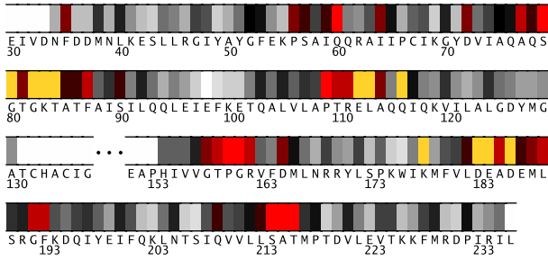
Fig. 1. Residues 30-236 in 3borA colored by their relative importance. (See Appendix, Fig.5, for the coloring scheme.)
