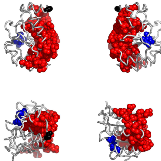
Fig. 2. Residues in 3borA, colored by their relative importance. Clockwise: front, back, top and bottom views.
