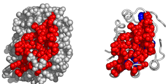
Fig. 4. A possible active surface on the chain 3borA. The larger cluster it belongs to is shown in blue.
