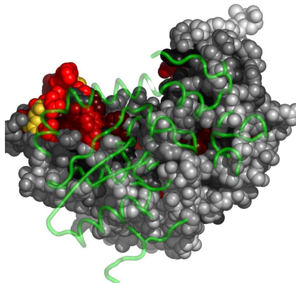
Fig. 5. Residues in 3c3jA, at the interface with 3c3jD, colored by their relative importance. 3c3jD is shown in backbone representation (See Appendix for the coloring scheme for the protein chain 3c3jA.)
