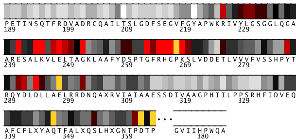
Fig. 2. Residues 189-384 in 3c3jA colored by their relative importance. (See Appendix, Fig.8, for the coloring scheme.)
