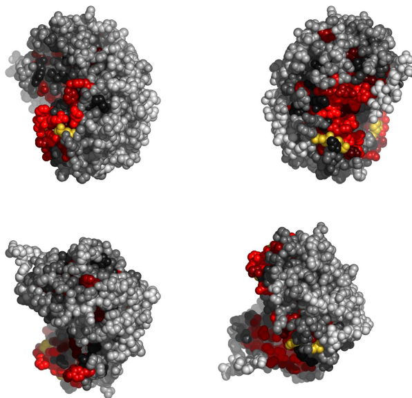
Fig. 3. Residues in 3c3jA, colored by their relative importance. Clockwise: front, back, top and bottom views.
