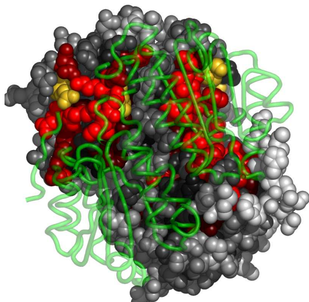
Fig. 6. Residues in 3c3jA, at the interface with 3c3jE, colored by their relative importance. 3c3jE is shown in backbone representation (See Appendix for the coloring scheme for the protein chain 3c3jA.)
