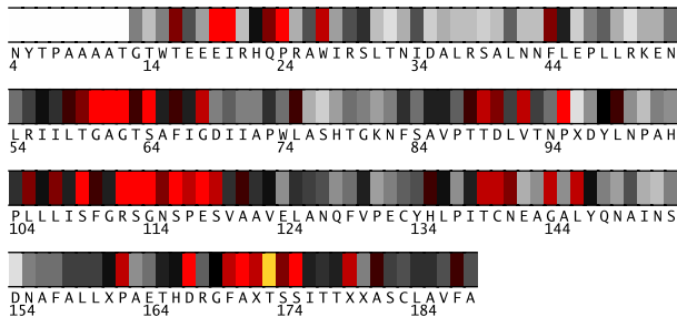
Fig. 1. Residues 4-188 in 3c3jA colored by their relative importance. (See Appendix, Fig.8, for the coloring scheme.)
