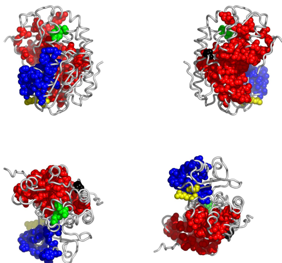
Fig. 4. Residues in 3c3jA, colored according to the cluster they belong to: red, followed by blue and yellow are the largest clusters (see Appendix for the coloring scheme). Clockwise: front, back, top and bottom views. The corresponding Pymol script is attached.
