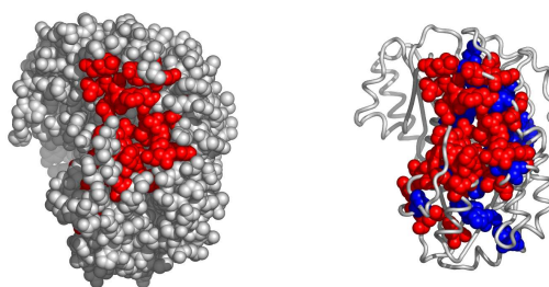
Fig. 7. A possible active surface on the chain 3c3jA. The larger cluster it belongs to is shown in blue.
