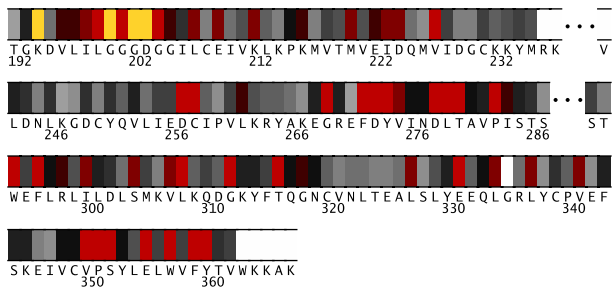
Fig. 2. Residues 192-367 in 3c6kA colored by their relative importance. (See Appendix, Fig.9, for the coloring scheme.)
