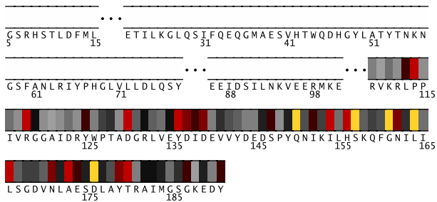
Fig. 1. Residues 5-191 in 3c6kA colored by their relative importance. (See Appendix, Fig.9, for the coloring scheme.)
