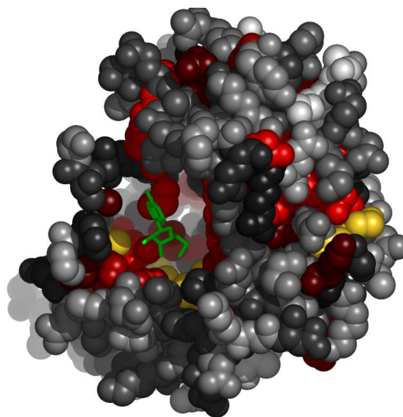
Fig. 7. Residues in 3c6kA, at the interface with MTA, colored by their relative importance. The ligand (MTA) is colored green. Atoms further than 30 Å away from the geometric center of the ligand, as well as on the line of sight to the ligand were removed. (See Appendix for the coloring scheme for the protein chain 3c6kA.)
