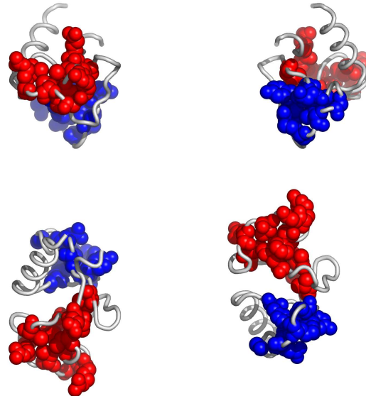
Fig. 3. Residues in 3d2nA, colored according to the cluster they belong to: red, followed by blue and yellow are the largest clusters (see Appendix for the coloring scheme). Clockwise: front, back, top and bottom views. The corresponding Pymol script is attached.
