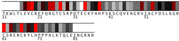
Fig. 1. Residues 11-86 in 3d2nA colored by their relative importance. (See Appendix, Fig.7, for the coloring scheme.)
