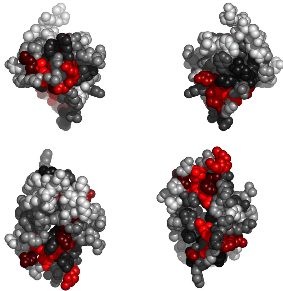
Fig. 2. Residues in 3d2nA, colored by their relative importance. Clockwise: front, back, top and bottom views.
