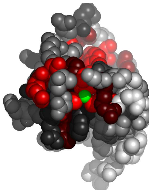
Fig. 4. Residues in 3d2nA, at the interface with zinc ion, colored by their relative importance. The ligand (zinc ion) is colored green. Atoms further than 30Å away from the geometric center of the ligand, as well as on the line of sight to the ligand were removed. (See Appendix for the coloring scheme for the protein chain 3d2nA.)
