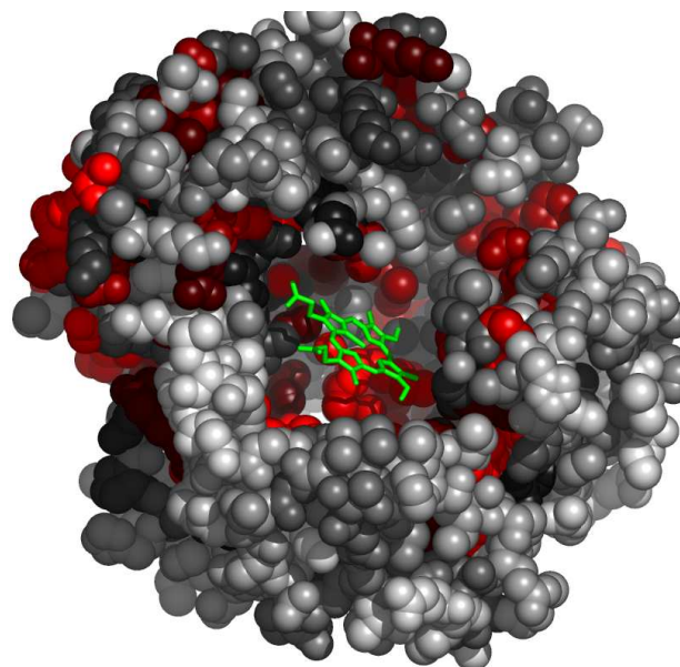
Fig. 6. Residues in 3daxA, at the interface with HEM, colored by their relative importance. The ligand (HEM) is colored green. Atoms further than 30Å away from the geometric center of the ligand, as well as on the line of sight to the ligand were removed. (See Appendix for the coloring scheme for the protein chain 3daxA.)
