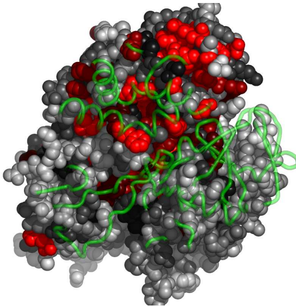
Fig. 5. Residues in 3daxA, at the interface with 3daxB, colored by their relative importance. 3daxB is shown in backbone representation (See Appendix for the coloring scheme for the protein chain 3daxA.)
