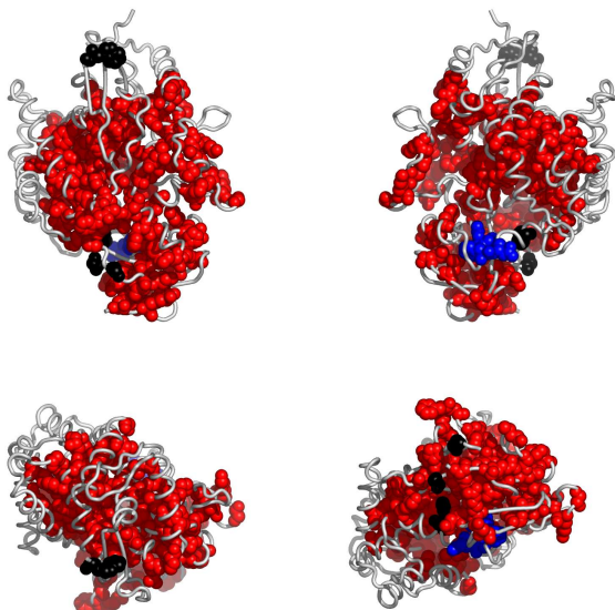
Fig. 4. Residues in 3daxA, colored according to the cluster they belong to: red, followed by blue and yellow are the largest clusters (see Appendix for the coloring scheme). Clockwise: front, back, top and bottom views. The corresponding Pymol script is attached.
