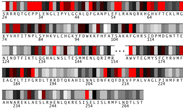
Fig. 1. Residues 24-269 in 3daxA colored by their relative importance. (See Appendix, Fig.8, for the coloring scheme.)
