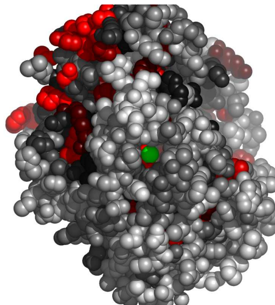
Fig. 7. Residues in 3daxA, at the interface with unknown atom or ion, colored by their relative importance. The ligand (unknown atom or ion) is colored green. Atoms further than 30Å away from the geometric center of the ligand, as well as on the line of sight to the ligand were removed. (See Appendix for the coloring scheme for the protein chain 3daxA.)
