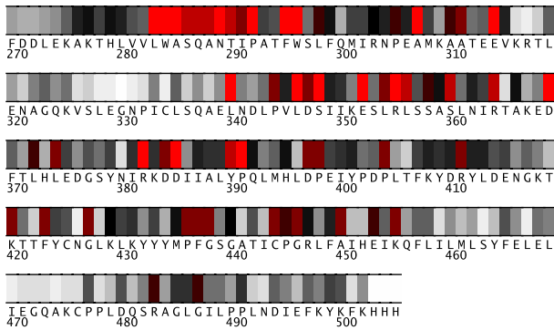
Fig. 2. Residues 270-505 in 3daxA colored by their relative importance. (See Appendix, Fig.8, for the coloring scheme.)
