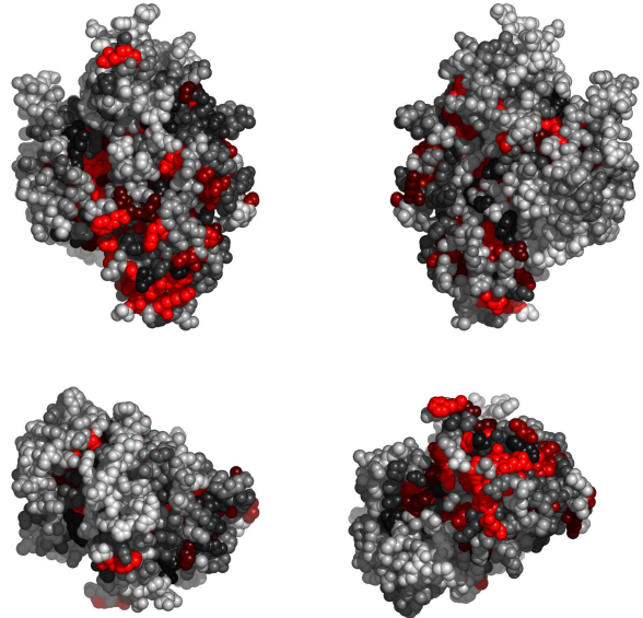
Fig. 3. Residues in 3daxA, colored by their relative importance. Clockwise: front, back, top and bottom views.
