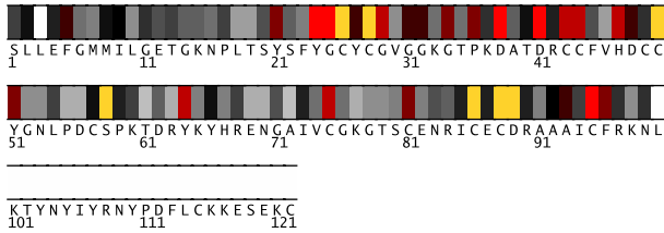
Fig. 1. Residues 1-122 in 3g8gA colored by their relative importance. (See Appendix, Fig.6, for the coloring scheme.)
