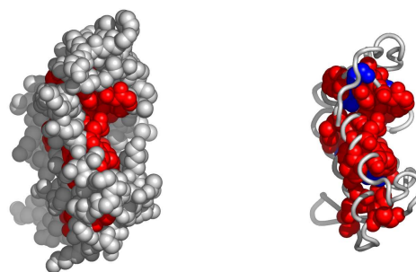
Fig. 5. A possible active surface on the chain 3g8gA. The larger cluster it belongs to is shown in blue.
