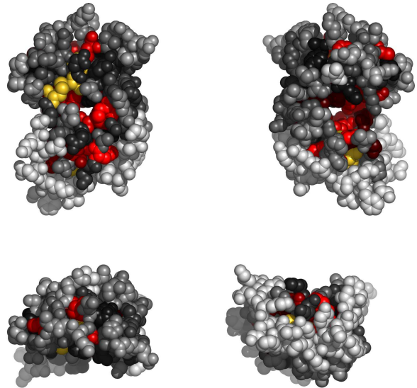
Fig. 1. Residues 1-122 in 3g8gA colored by their relative importance. (See Appendix, Fig.6, for the coloring scheme.)
