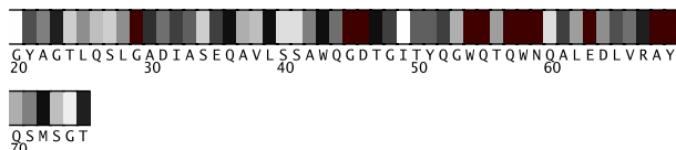
Fig. 4. Residues 20-75 in 3h6pC colored by their relative importance. (See Appendix, Fig.11, for the coloring scheme.)
