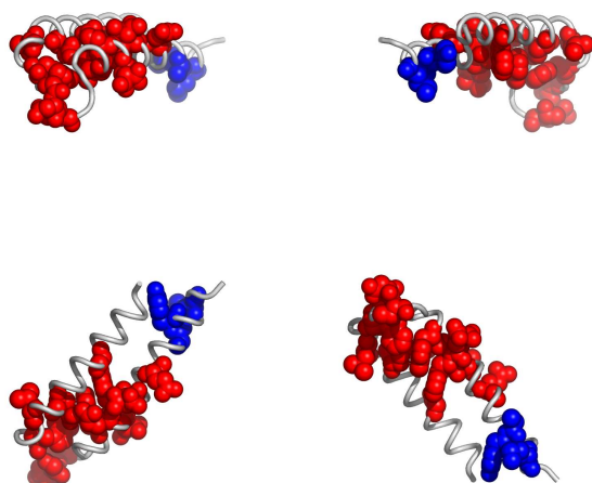
Fig. 6. Residues in 3h6pC, colored according to the cluster they belong to: red, followed by blue and yellow are the largest clusters (see Appendix for the coloring scheme). Clockwise: front, back, top and bottom views. The corresponding Pymol script is attached.
