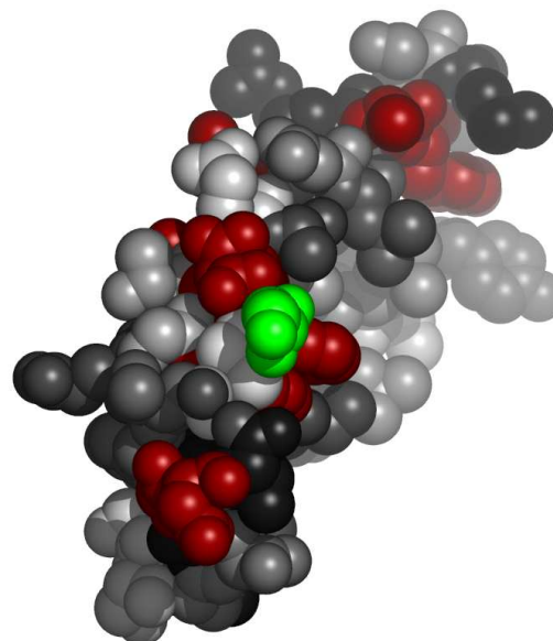
Fig. 7. Residues in 3h6pC, at the interface with glycerol, colored by their relative importance. The ligand (glycerol) is colored green. Atoms further than 30 Å away from the geometric center of the ligand, as well as on the line of sight to the ligand were removed. (See Appendix for the coloring scheme for the protein chain 3h6pC.)
