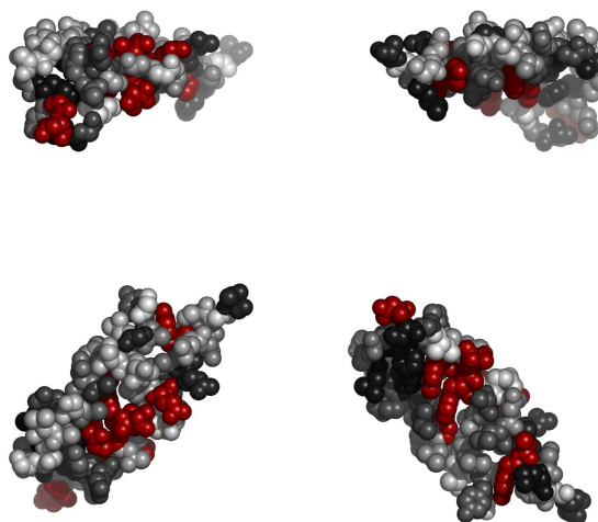
Fig. 5. Residues in 3h6pC, colored by their relative importance. Clockwise: front, back, top and bottom views.
