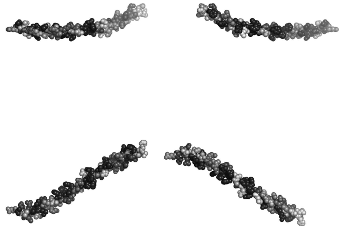
Fig. 1. Residues 14-80 in 3h6pB colored by their relative importance. (See Appendix, Fig.11, for the coloring scheme.)
