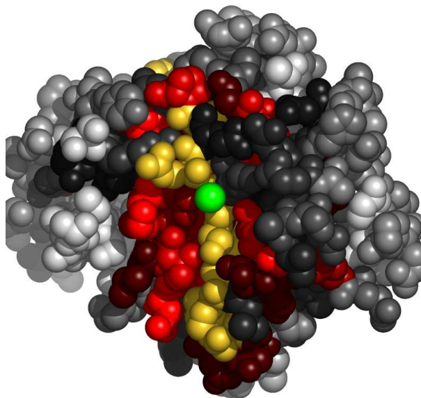
Fig. 4. Residues in 3iugB, at the interface with unknown atom or ion, colored by their relative importance. The ligand (unknown atom or ion) is colored green. Atoms further than 30 Å away from the geometric center of the ligand, as well as on the line of sight to the ligand were removed. (See Appendix for the coloring scheme for the protein chain 3iugB.)
