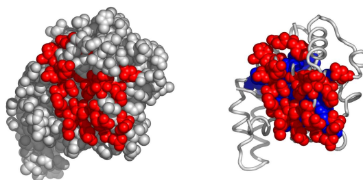
Fig. 9. A possible active surface on the chain 3iugB. The larger cluster it belongs to is shown in blue.
