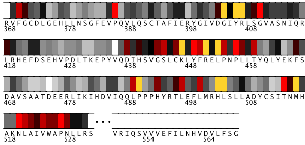
Fig. 1. Residues 368-569 in 3iugB colored by their relative importance. (See Appendix, Fig.10, for the coloring scheme.)
