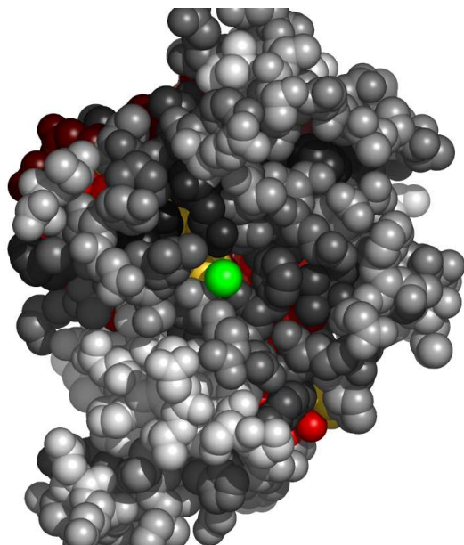
Fig. 5. Residues in 3iugB, at the interface with unknown atom or ion, colored by their relative importance. The ligand (unknown atom or ion) is colored green. Atoms further than 30Å away from the geometric center of the ligand, as well as on the line of sight to the ligand were removed. (See Appendix for the coloring scheme for the protein chain 3iugB.)
