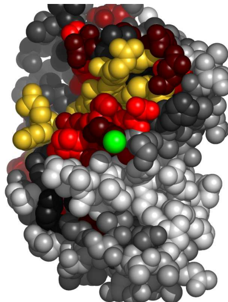
Fig. 7. Residues in 3iugB, at the interface with unknown atom or ion, colored by their relative importance. The ligand (unknown atom or ion) is colored green. Atoms further than 30Å away from the geometric center of the ligand, as well as on the line of sight to the ligand were removed. (See Appendix for the coloring scheme for the protein chain 3iugB.)
