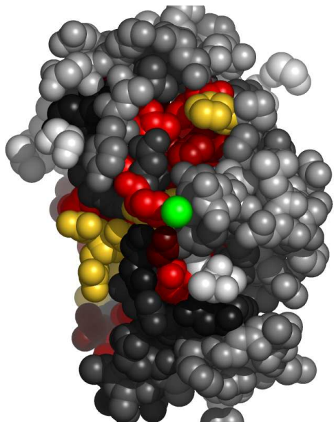
Fig. 6. Residues in 3iugB, at the interface with unknown atom or ion, colored by their relative importance. The ligand (unknown atom or ion) is colored green. Atoms further than 30Å away from the geometric center of the ligand, as well as on the line of sight to the ligand were removed. (See Appendix for the coloring scheme for the protein chain 3iugB.)
