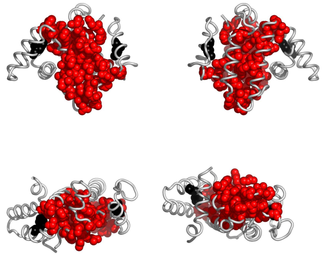
Fig. 2. Residues in 3iugB, colored by their relative importance. Clockwise: front, back, top and bottom views.
