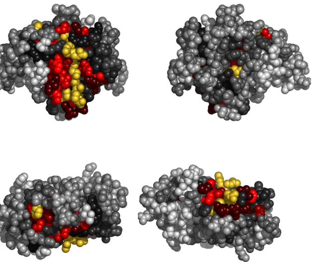
Fig. 2. Residues in 3iugB, colored by their relative importance. Clockwise: front, back, top and bottom views.
