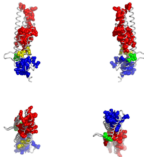
Fig. 3. Residues in 3ljbA, colored by their relative importance. Clockwise: front, back, top and bottom views.
