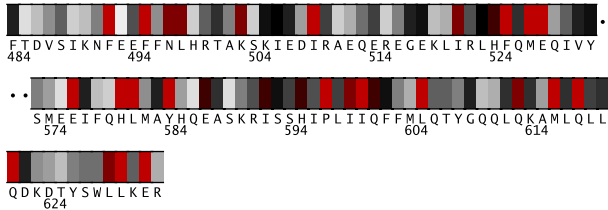
Fig. 2. Residues 484-633 in 3ljbA colored by their relative importance. (See Appendix, Fig.9, for the coloring scheme.)
