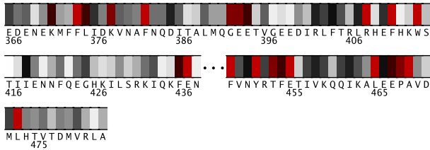
Fig. 1. Residues 366-483 in 3ljbA colored by their relative importance. (See Appendix, Fig.9, for the coloring scheme.)
