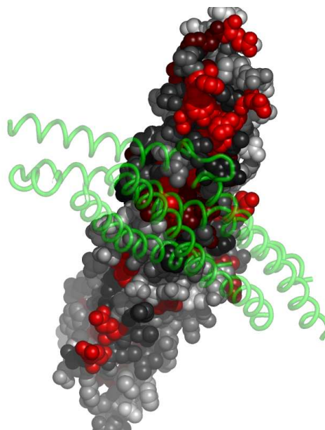
Fig. 5. Residues in 3ljbA, at the interface with 3ljbB, colored by their relative importance. 3ljbB is shown in backbone representation (See Appendix for the coloring scheme for the protein chain 3ljbA.)
