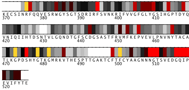
Fig. 1. Residues 370-526 in 3no8A colored by their relative importance. (See Appendix, Fig.8, for the coloring scheme.)
