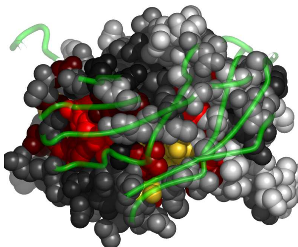
Fig. 4. Residues in 3no8A, at the interface with 3no8B, colored by their relative importance. 3no8B is shown in backbone representation (See Appendix for the coloring scheme for the protein chain 3no8A.)
