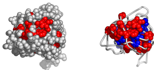
Fig. 7. A possible active surface on the chain 3no8A. The larger cluster it belongs to is shown in blue.
