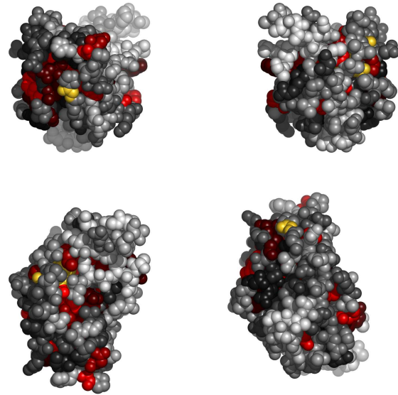
Fig. 2. Residues in 3no8A, colored by their relative importance. Clockwise: front, back, top and bottom views.
