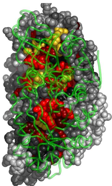
Fig. 6. Residues in 70dcA, at the interface with 70dcA1, colored by their relative importance. 70dcA1 is shown in backbone representation (See Appendix for the coloring scheme for the protein chain 70dcA.)
