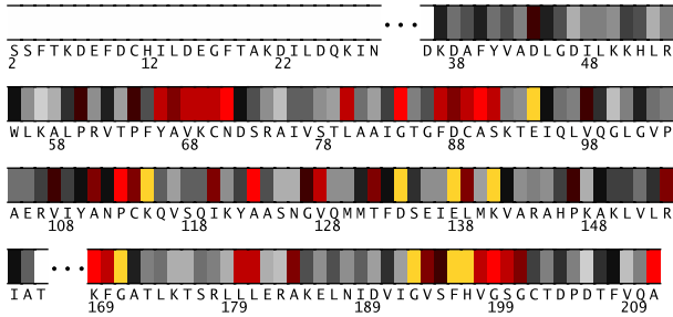
Fig. 1. Residues 2-211 in 7odcA colored by their relative importance. (See Appendix, Fig.8, for the coloring scheme.)
