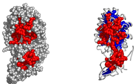
Fig. 7. A possible active surface on the chain 70dcA. The larger cluster it belongs to is shown in blue.
