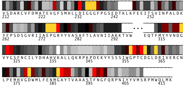
Fig. 2. Residues 212-418 in 7odcA colored by their relative importance. (See Appendix, Fig.8, for the coloring scheme.)
