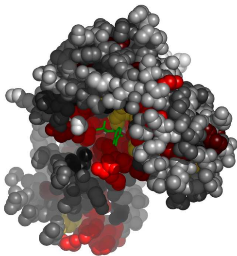
Fig. 5. Residues in 7odcA, at the interface with PLP, colored by their relative importance. The ligand (PLP) is colored green. Atoms further than 30Å away from the geometric center of the ligand, as well as on the line of sight to the ligand were removed. (See Appendix for the coloring scheme for the protein chain 7odcA.)
